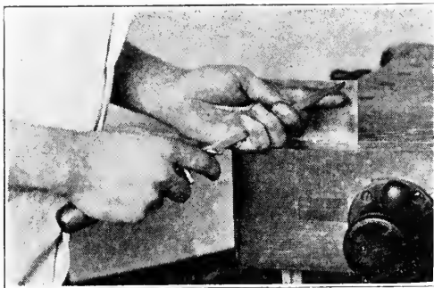
FIG. 121. RAISING BURR ON SCRAPER.
